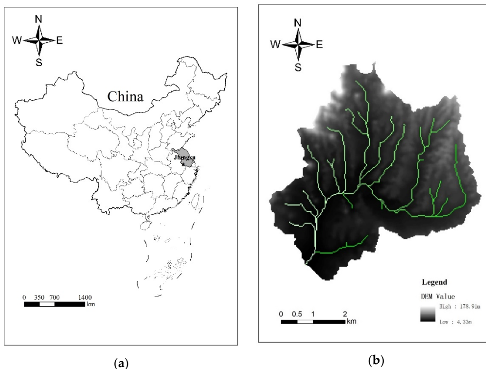
Figure 2. (a) Location of Peiqiao River watershed in China; (b) DEM feature of Peiqiao River watershed.
