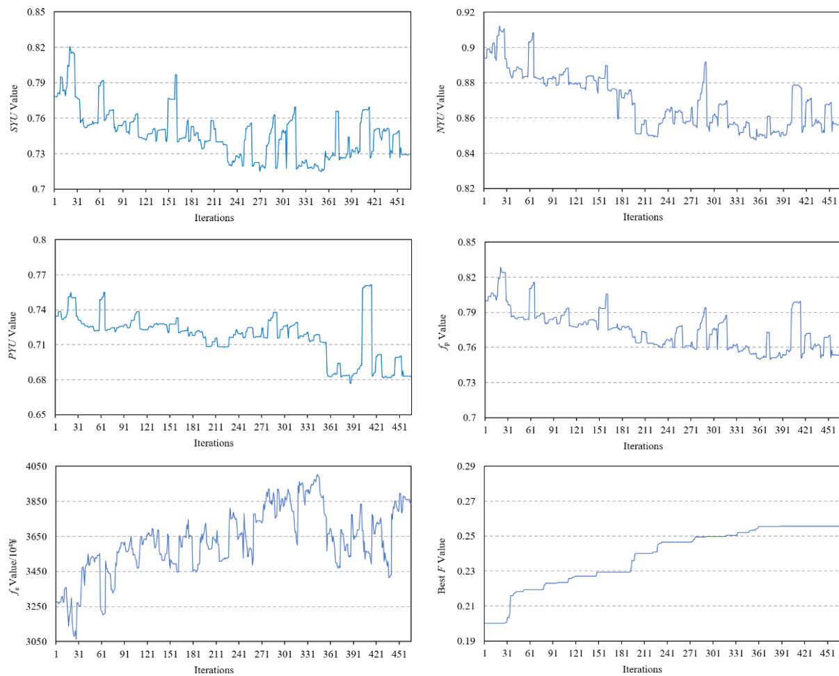
Figure 4. The value of each objective function changed with the MTSA iteration.
